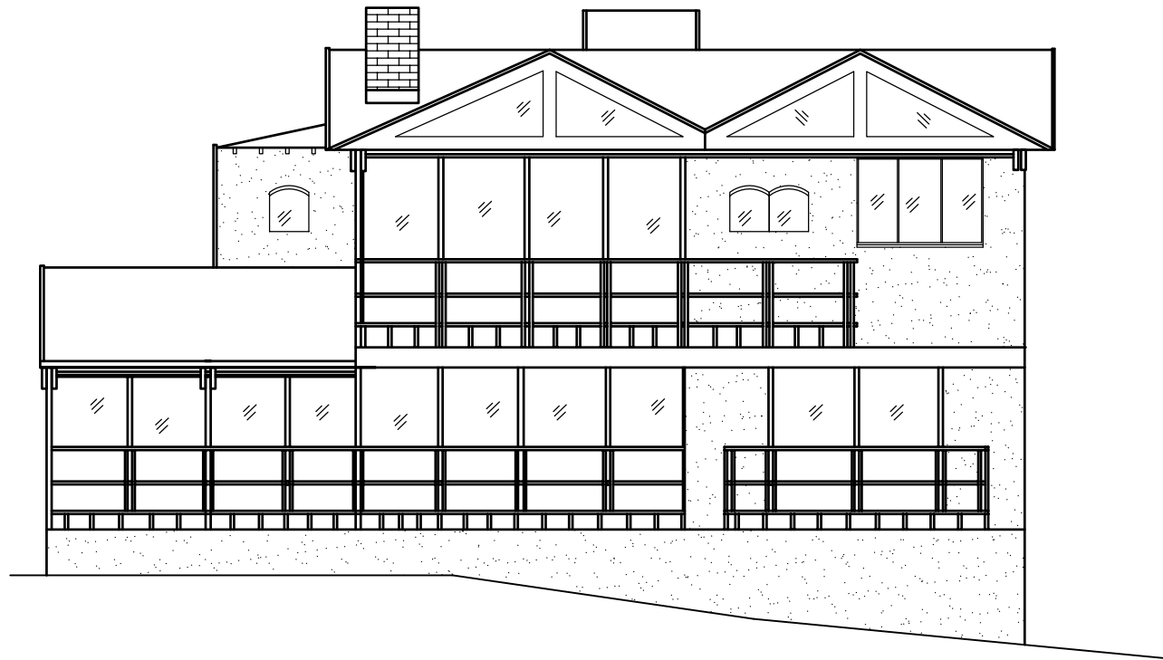
SOUTHEAST ELEVATION
