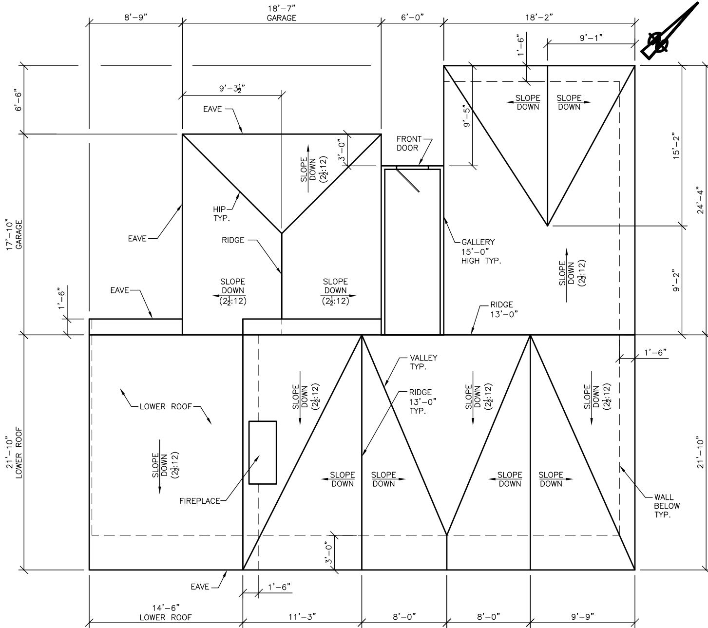
NEW ROOF PLAN
