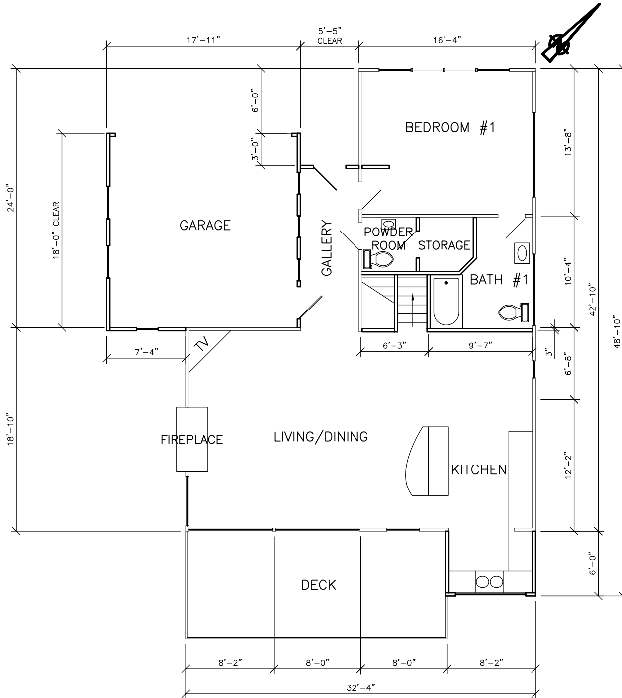
NEW PLAN - UPPER FLOOR
