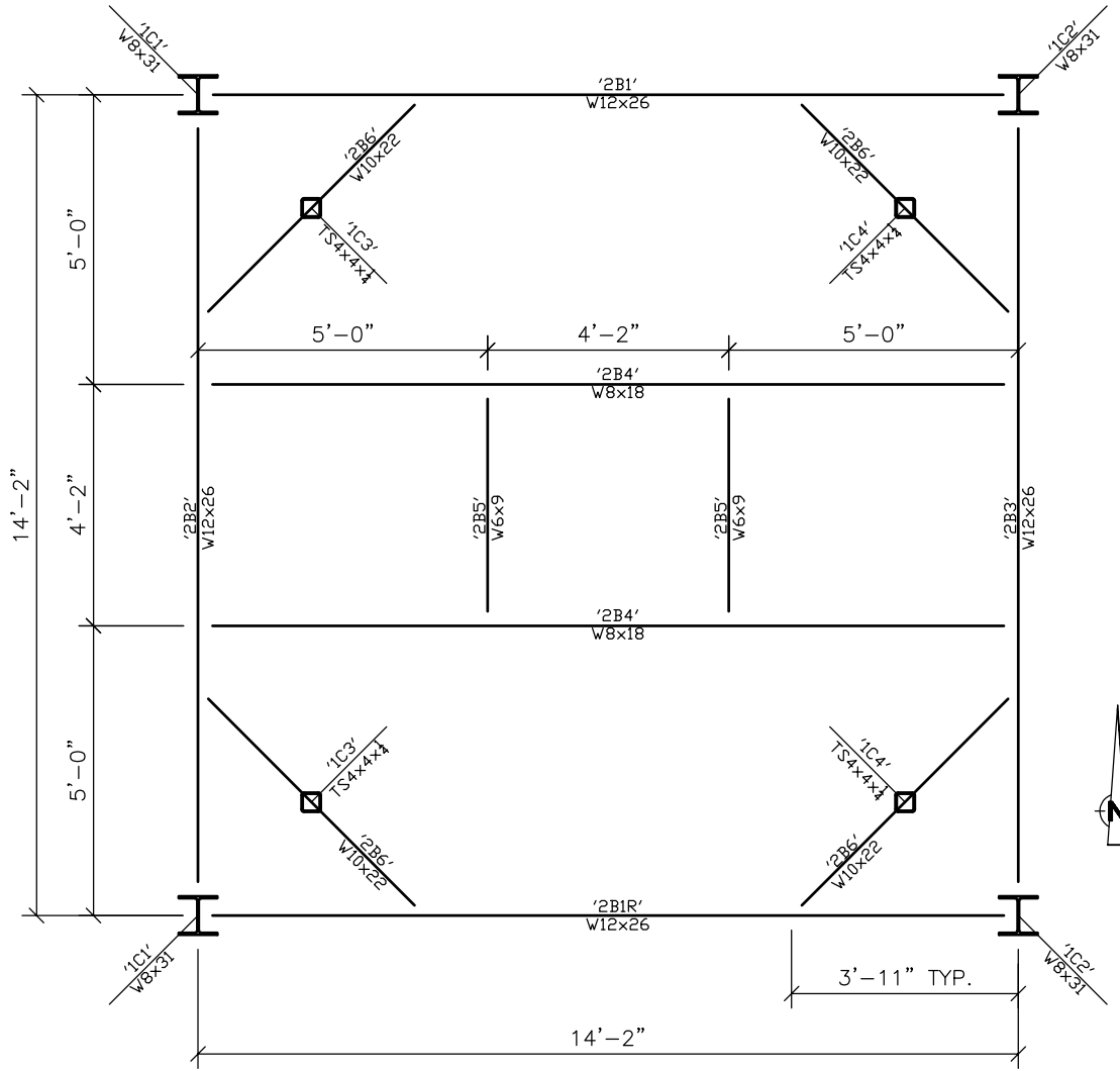
STEEL FRAMING PLAN
